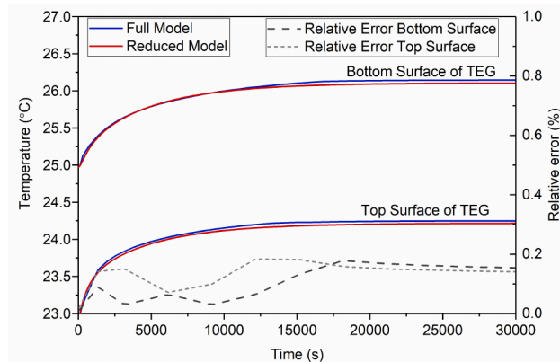
Figure 5: Temperature result of the full and the reduced model at the bottom and top surfaces of a TEG with muscle tissue divided into ten segments.
