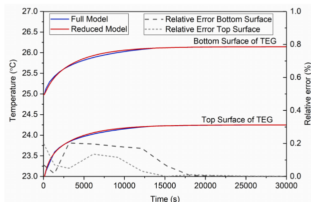
Figure 6: Temperature result for the full and reduced model at the bottom and top surfaces of a TEG with muscle tissue divided into fifteen segments.
