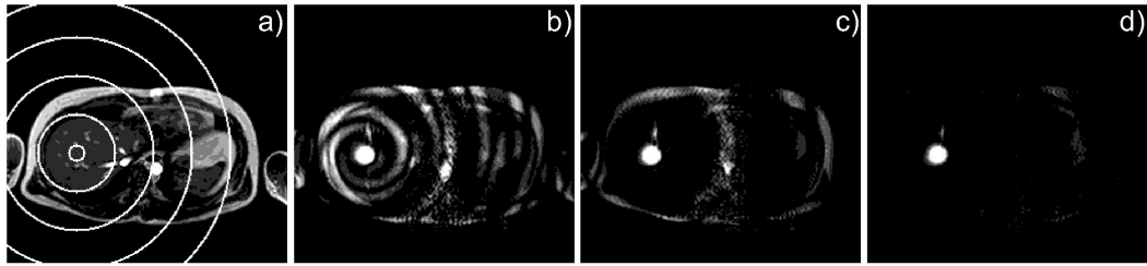
Figure 3. Transversal spin-echo images of the pencil beam excitation in the abdominal region (b-d). In the transversal survey (a) the expected positions of the central beam and the aliasing rings for a 3-turn spiral are indicated by white circles. With increasing number of k-space turns (b-d: 3,6,12) the rings are shifted out of the body. The corresponding pulse lengths are 1.7ms, 2.8 ms, and 5.7 ms, respectively.
