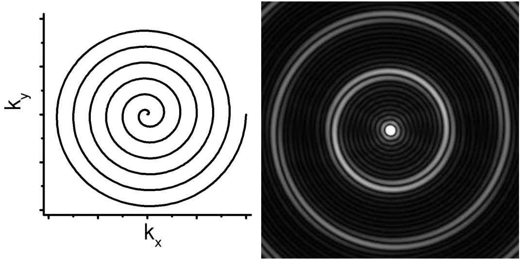
Figure 2. Spiral trajectory of 2D-RF pulse (left) and corresponding point spread function (right). The aliasing rings appear due to the discrete k -space covering of the spiral. The central peak is used as a pencil beam navigator.
