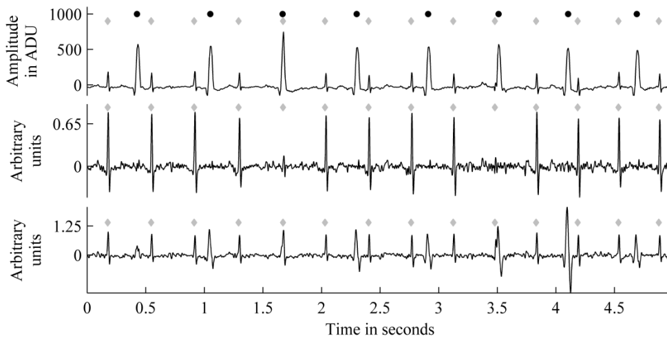
Figure 4. Simulated abdominal recording (SNR = -9 dB) (topmost signal) with its fetal component as extracted by means of KF (middle signal) and ESC (lowermost signal). Existing maternal (in the topmost signal) and fetal QRS complexes (in all signals) are marked by black circles and gray diamonds, respectively.
